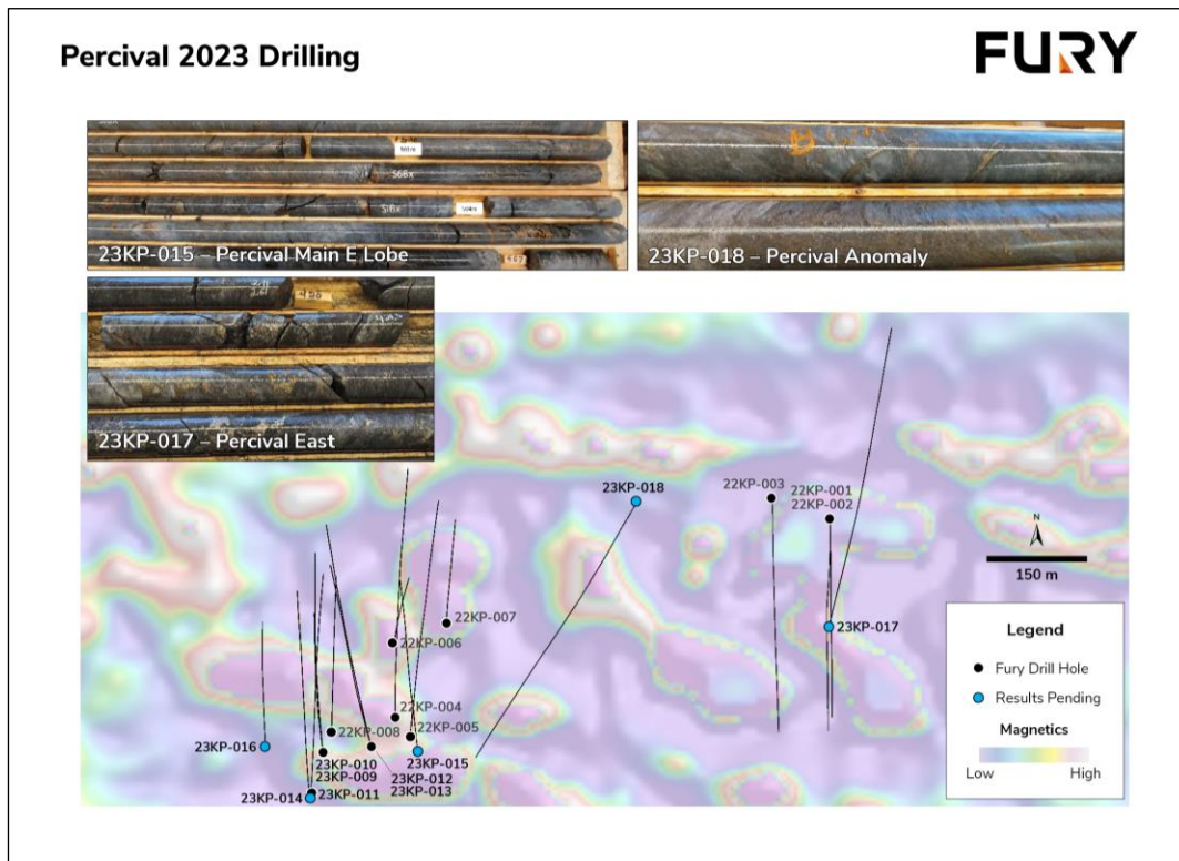
Figure 2: Plan view of the Percival Trend showing the two drill holes testing the prioritized biogeochemical anomalies in relation to 2023, 2022 and historical drill intercepts.
