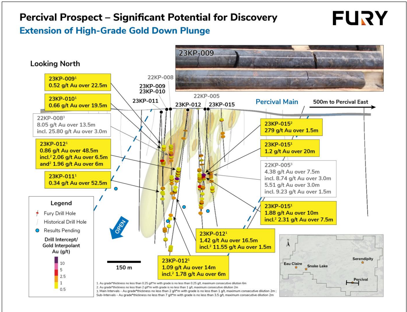
Figure 1: Percival long section depicting the locations of the current and pending 2023 drill holes in relation to the 2022 and historical drill intercepts.
