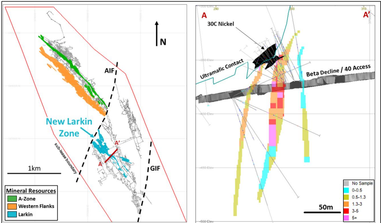
Figure 2(A): Beta Hunt Gold Resource plan highlighting location of new Larkin Zone Mineral Resource; Figure 2A: Cross-section through central Larkin Zone showing resource block model with gold grades
