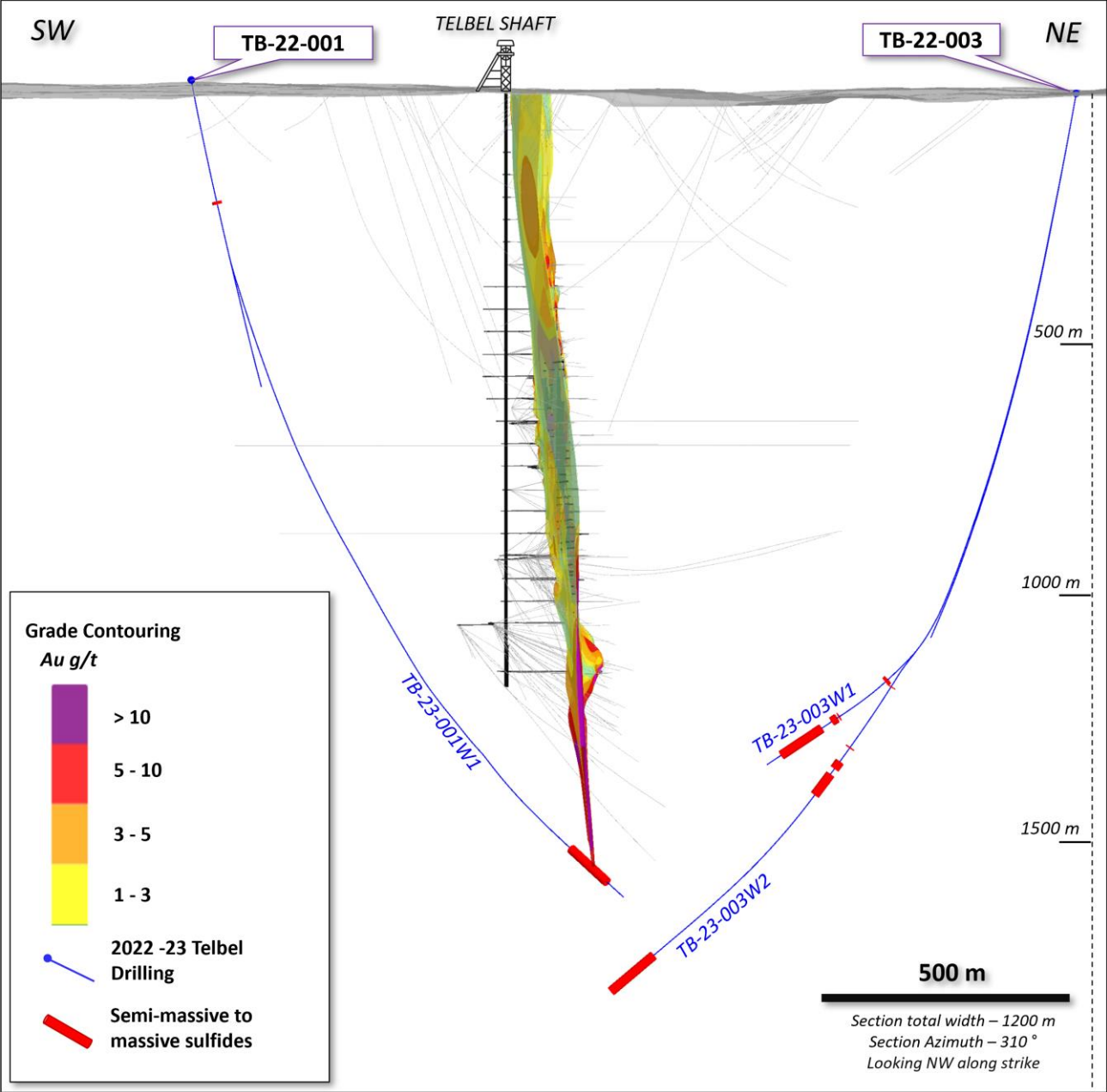
Figure 1: Section view showing master and wedge traces for two (2) of the three (3) drill holes
