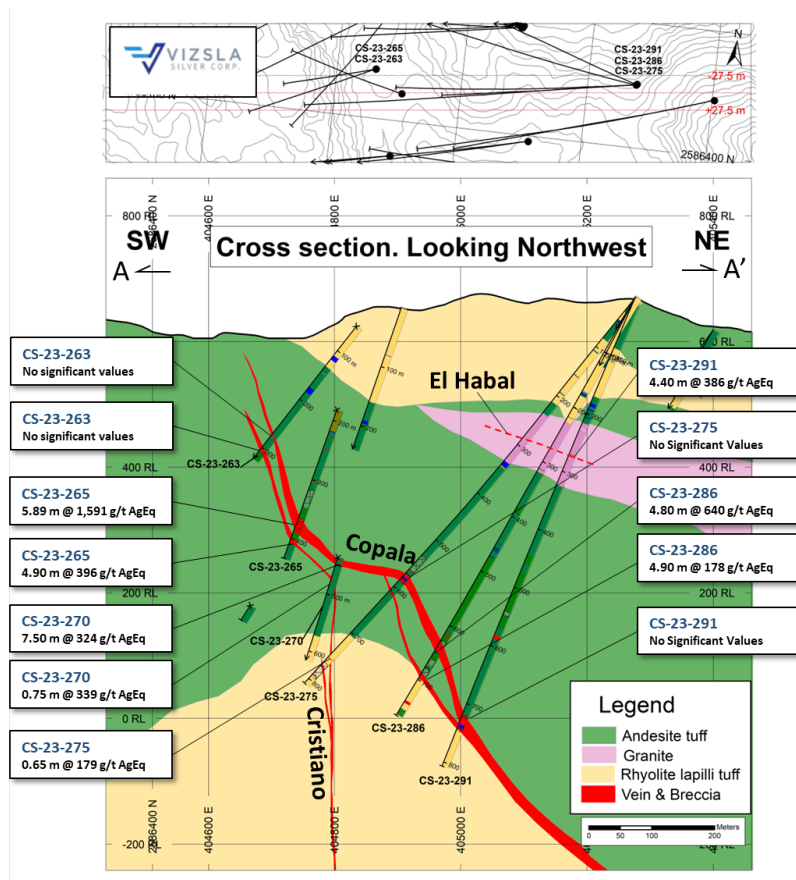
Figure 3: Cross section showing Copala structure and Cristiano vein with completed drilling.
