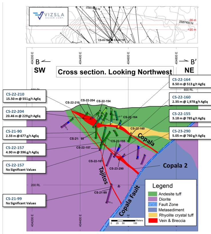
Figure 5: Cross section showing Copala 2, Copala and Tajitos veins with completed drilling.
