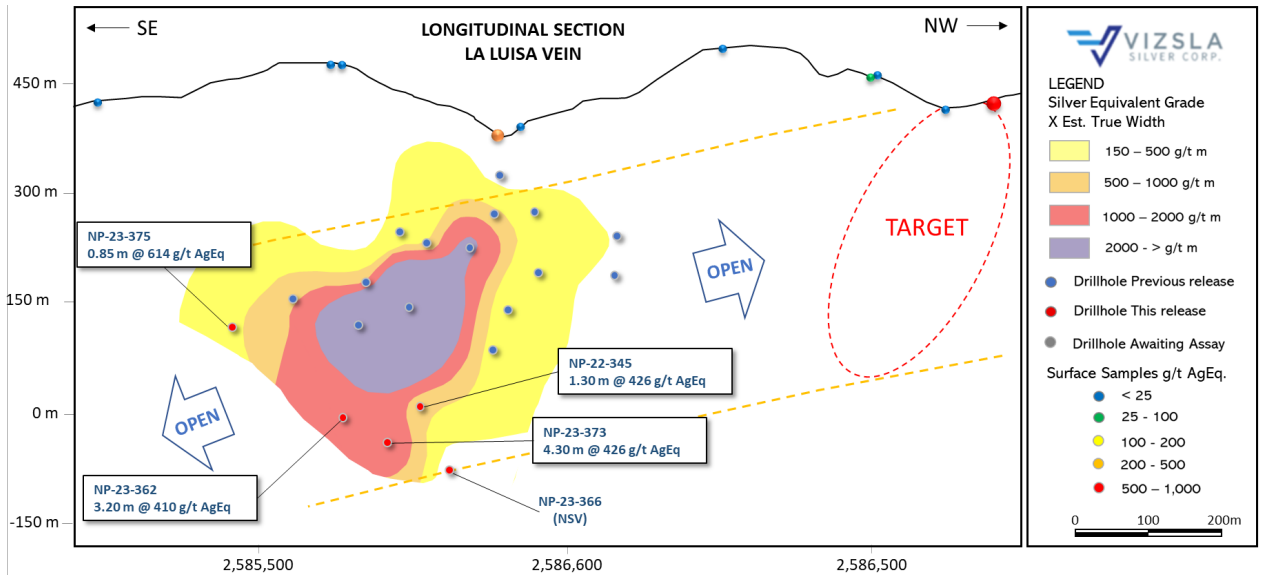
Figure 2: Longitudinal section of the La Luisa Vein.
