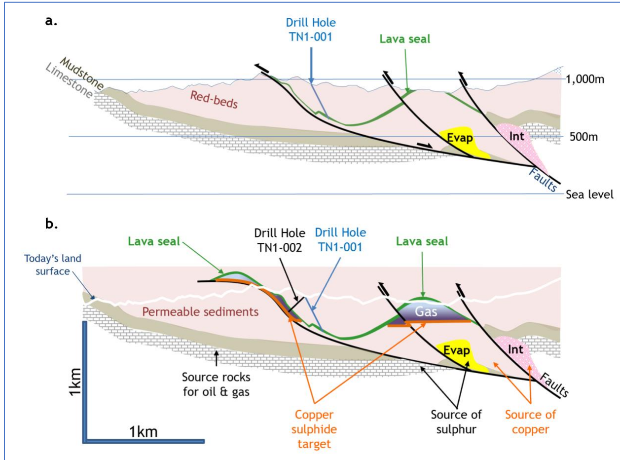
Figure 2a. Vertical profile through drill hole TN1-001 that intersected native copper beneath the lava layer (shown in green). b. Shows the structure of the profile as it is likely to have been before today's erosion level. Oil and gas are likely to have accumulated in the top of the fold arches. (Evap. is evaporite, a mixture of salt and sulphate minerals. Int. is intrusive, potentially copper-bearing porphyries).
