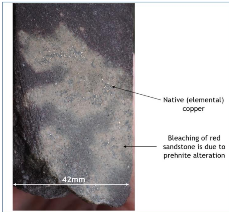
Figure 1. Native copper in bleached zones in core from the Tsenken N1 target.
