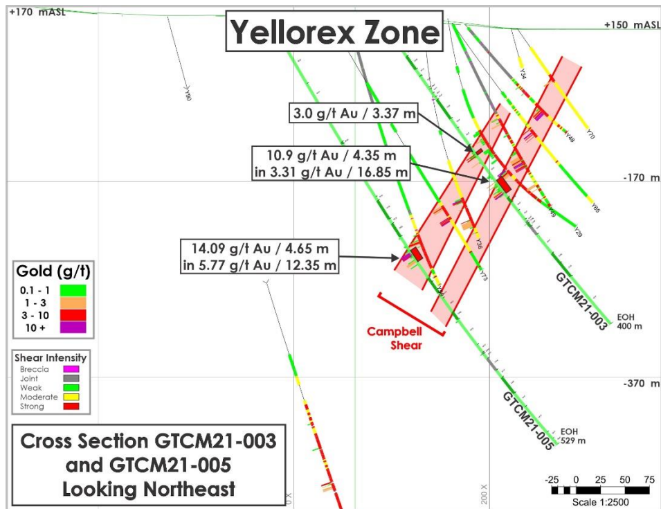
Figures 3 – Drill hole cross-section
