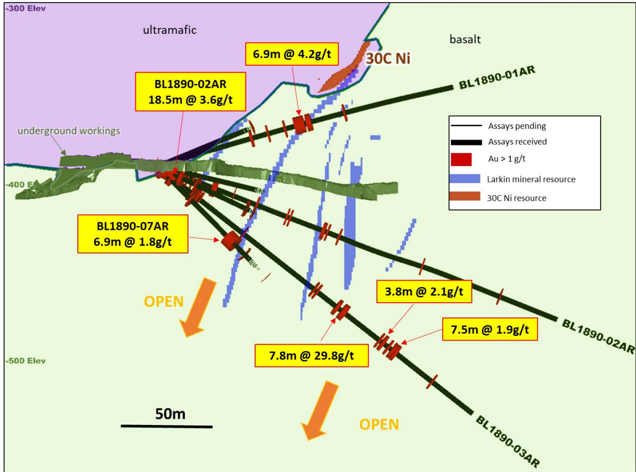
Figure 2: Larkin Zone cross section looking northwest with Larkin Mineral Resource and highlighted recent drill results.
