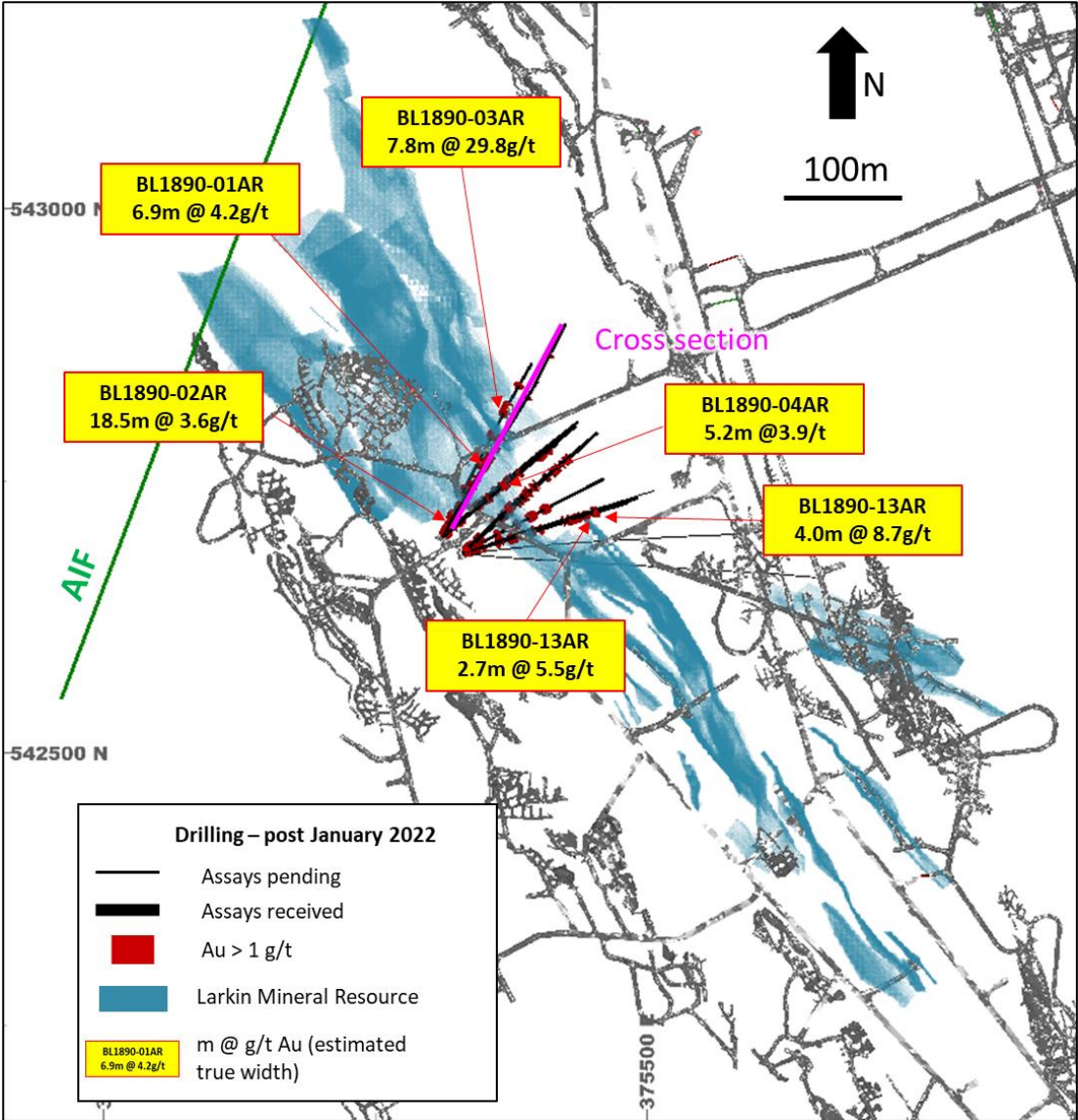
Figure 1: Beta Hunt plan view with Larkin Mineral Resource and highlighted recent drill results
