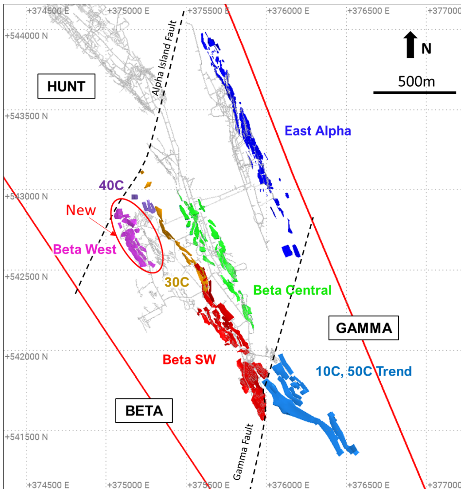
Figure 1: Beta Hunt plan view showing locations of the Beta Hunt nickel Mineral Resource
